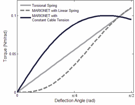
Fig. 3. Torque-deflection curve using rotational constraint compared to torsional spring. The torque-deflection curves from the rotational constraints in Figure 2 show a sinusoidal relationship, differing from the linear relationship of a torsional spring. Note that a linear spring results in a decrease of sensitivity to deflection, while constant tension results in an increase of sensitivity. Typical values for R_L (0.3 m), R_P (0.1 m), cable tension of 10 N, and spring constant (10 N/m) were used in the calculations.
