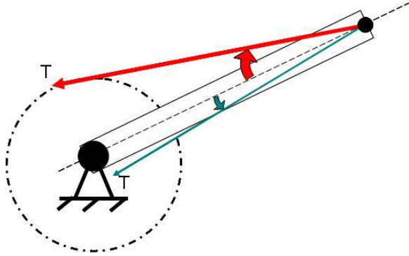
Fig. 2. Larger moment arms exert more torque. Two cases are shown in this illustration: The thick red arrow presents the case of a larger moment arm, which results in more torque, and the blue arrow exhibits the opposite case. The tension is the same in both cases. Also note that zero torque occurs when the arrow passes through the joint center.
