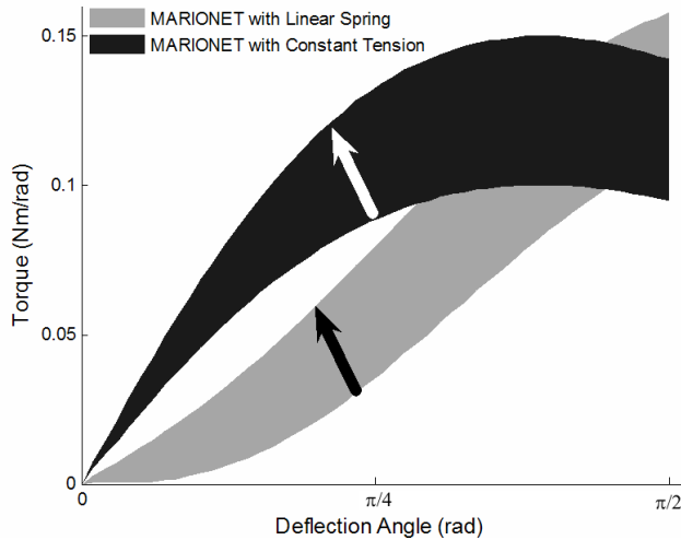
Fig. 4. Pretensioning acts as compliance control The MARIONET is capable of both equilibrium point and compliance control, all done mechanically. The Tensioner acts as a gain for compliance. Typical pretensioning values range from 0 to 5 cm for the 10 N/m spring, and 1 to 1.5 N for cable tension.
