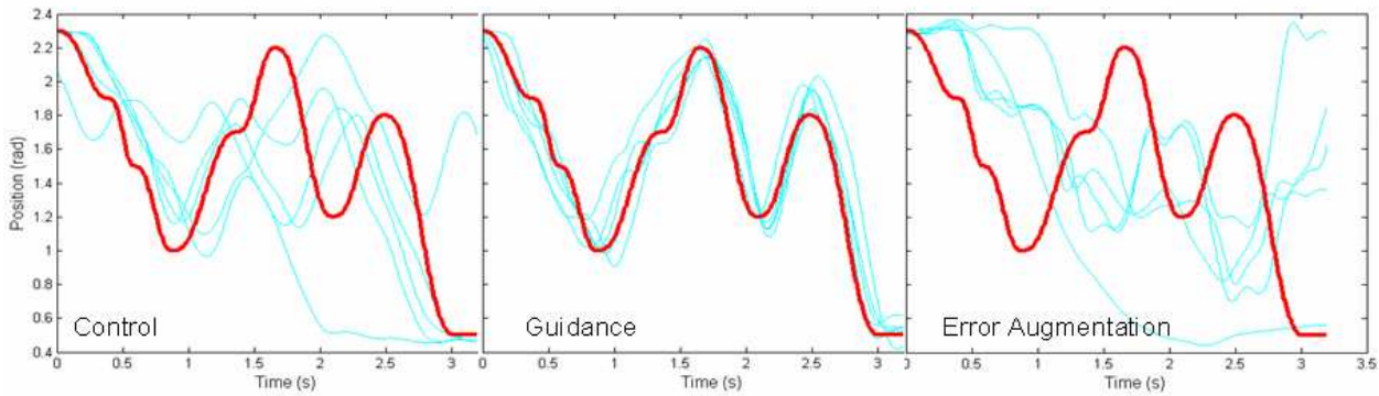
Fig. 6. Results of pilot experiment. Red lines show desired trajectory, and blue lines show the individual trials. Qualitatively, it seems that the MARIONET is capable of exerting a trajectory on its user even though it is a torque controlled device. Since the device itself has no damping, it depends on the damping of the user for stability.
